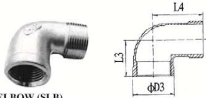
90° 内外牙弯头 STREET ELBOW (SLB)
