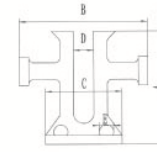
Cross Bollard
