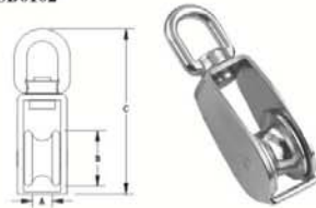
SANMA SWIVEL BLOCK (STAINLESS SHEAVE WITH BRASS BUSHING), SS304 OR SS316.
