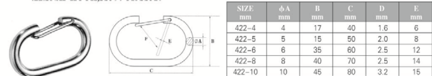
422.SNAP HOOK,SS304 OR SS316
