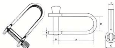
PLATE DEE SHACKLE,SS304 OR SS316 CSXK0702
