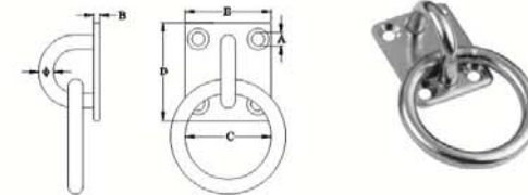
SQUARE EYE PLATE WITH RING,SS304 OR SS316. CSMK02
