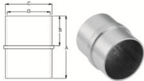
BALUSTRADE SOCKET, SS304 OR SS316
