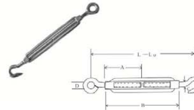
EU CLOSED BODY TURNBUCKLE(欧式封闭花兰螺丝) CSHL03FJ
