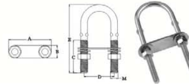
U-BOLT WITH WASHER AND NUTS,SS304 OR SS316.
