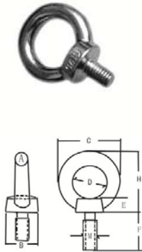
EYE BOLT DIN580,CSL502
