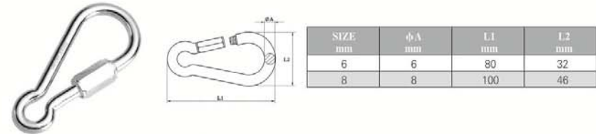
FLAT SNAP HOOK WITH TWO RIVETS,SS304 OR SS316
