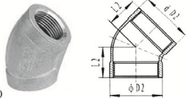
45° 弯头 45° ELBOW (45LB)
