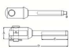
TOGGLE TERMINAL,SS304 OR SS316. CSJX06
