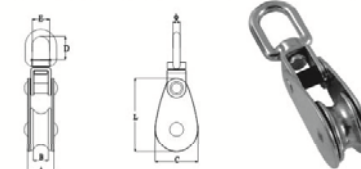
MAME SWIVEL BLOCK(STAINLESS CASTING SHEAVE),SS304 OR SS316.
