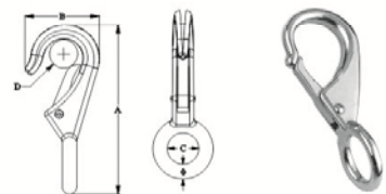
RIGID EYE SNAP,SS304 OR SS316. CSSH06
