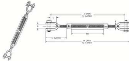
JAW & JAW TURNBUCKLES HG-228, SS304 OR SS316.
