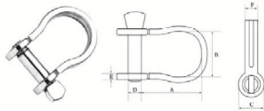
PLATE BOW SHACKLE,SS304 OR SS316 CSXK0701
