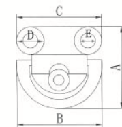
Folding Pad eye
