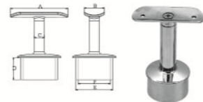
RAIL BRACKET 2" TUBE TOP MOUNT SQUARE, SS304 OR SS316
