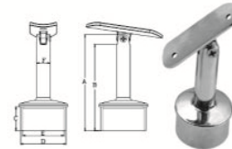
RAIL BRACKET 2" TUBE TOP MOUNT ADJUSTABLE, SS304 OR SS316
