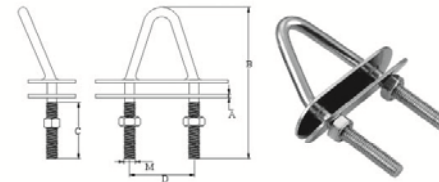
V-BOLT WITH WASHER AND NUTS,SS304 OR SS316. CSUS
