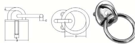
ROUND EYE PLATE WITH RING,SS304 OR SS316.CSMK08
