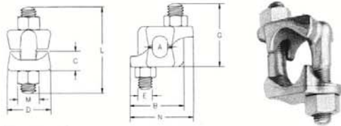
WIRE ROPE END TERMINATIONS,SS304 OR SS316 . CSKT08
