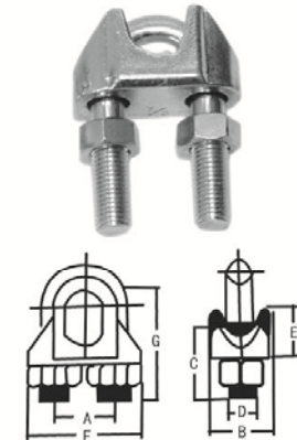
TYPE MALLEABLE WIRE ROPE CLIPS(美式玛钢型卡头) CSKT04
