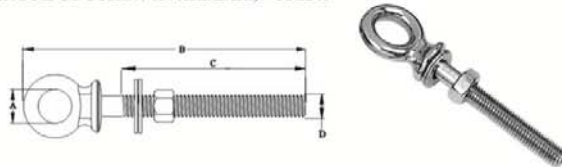
EYE BOLT, SS316 (ANY LENGTH OF SCREW AVAILABLE). CSLS03
