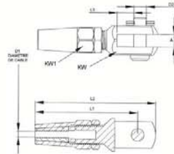
SWAGELESS THREAD TERMINAL, SS304 OR SS316. CSJX18
