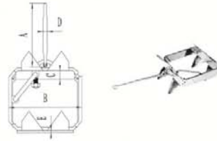
Stainless Steel and Carbon Steel Square Anchor 四方锚
