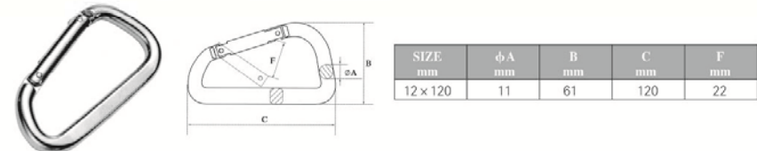
SNAP HOOK WITH BAR,SS304 OR SS316
