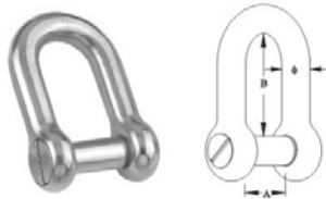
D-SHACKLE (WITH SLOT SINK PIN),SS304 OR SS316
