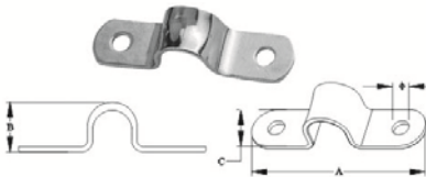
EYE STRAP(TWO HOLE TYPE),SS304 OR SS316.CSLB02
