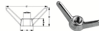
WING NUT(LONG TYPE),SS304 OR SS316. CSLM040L
