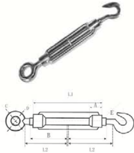
TURNBUCKLE DIN1480(SS304 OR SS316) CSHL05HE
