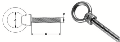
EYE BOLT, SS316 (ANY LENGTH OF SCREW AVAILABLE). SS304 OR SS316. CSL501
