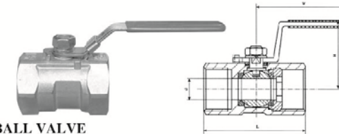
一片式球阀 1-PC BALL VALVE
