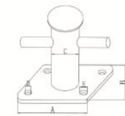
Cross Bollard Single 单十字缆桩
