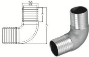
CGWT01 HOSE FITTING 90° , SS304 OR SS316
