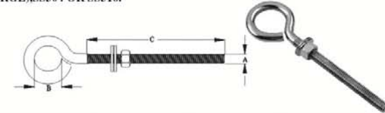
EYE BOLT (FORGE), SS304 OR SS316.
