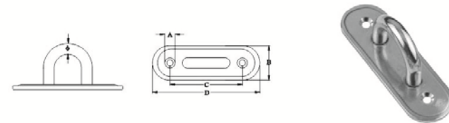
OVAL EYE PLATE,SS304 OR SS316. CSMK03
