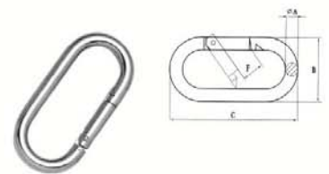
STRAIGHT SNAP HOOK WITH SCREW,SS304 OR SS316,STEEL ELECTRIC GALVANIZED
