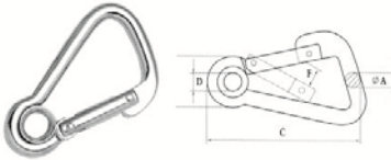
SWIVEL EYE SNAP,SS304 OR SS316. CSSH05
