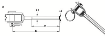
FORK TERMINAL FORGED, SS304 OR SS316. CSJX02
