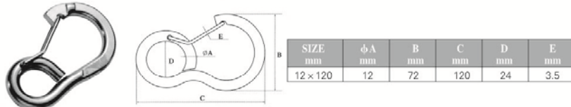
DELTA SNAP HOOK,SS304 OR SS316
