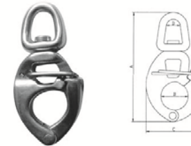
SNAP HOOK WITH EYE,SS304 OR SS316
