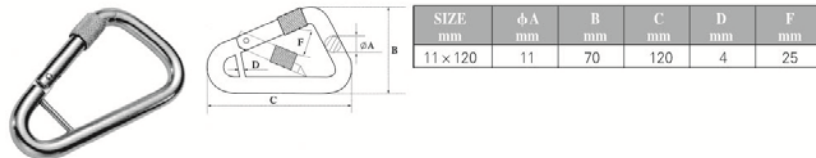
DELTA SNAP HOOK WITH SCREW AND BAR,SS304 OR SS316
