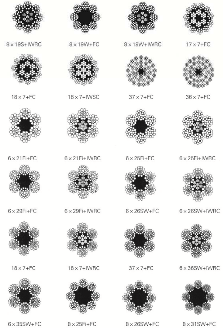
钢丝绳典型结构 Typical Rope Constructions
