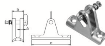
DECK HINGE (CONCAVE BASE WITH REMOVABLE PIN),SS304 OR SS316.
