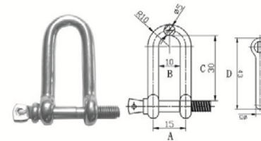
SHACKLE WITH LONGER THREAD
