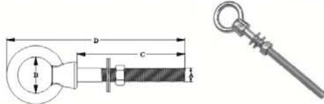
LIFTING EYE BOLT WITH DOUBLE WASHER AND NUT, SS304 OR SS316. CSL501
