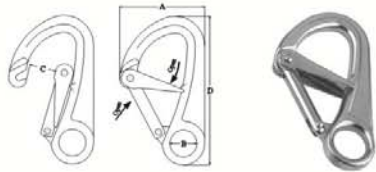
SPRING HOOK CASTING,SS304 OR SS316.
