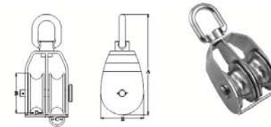
MAME SWIVEL BLOCK(DOUBLE CASTING SHEAVE WITH EYE END),SS304 OR SS316.
