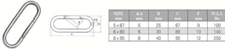
D TYPE SNAP HOOK STEEL ELECTRIC CALVANIZED
