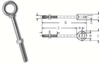
US EYE BOLT G-277 (美式吊环螺丝 G-277)
