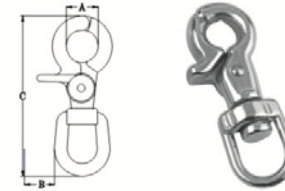
SWIVEL EYE BOLT SNAP,SS304 OR SS316. CSSH01
