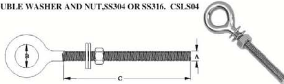
WIRE EYE BOLT WITH DOUBLE WASHER AND NUT, SS304 OR SS316. CSLS04
