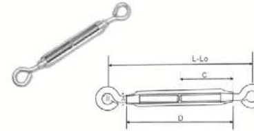
EU TYPE TURNBUCKLE(欧式开体花兰螺丝) CSHL03EH
