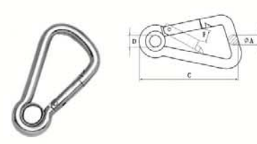
STRAIGHT SNAP HOOK,SS304 OR SS316,STEEL ELECTRIC GALVANIZED
