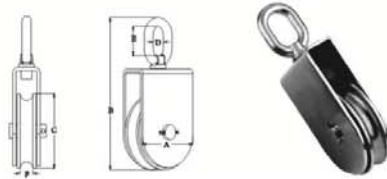
SANMA SWIVEL BLOCK (STAINLESS SHEAVE WITH BRASS BUSHING), SS304 OR SS316.
