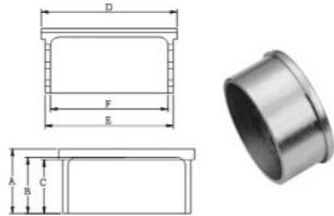
BALUSTRADE MAST TOP PLUG, SS304 OR SS316
