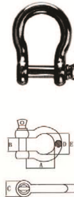
BOW SHACKLE
