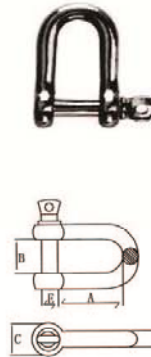
DEE SHACKLE
