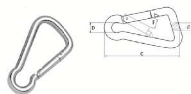
OBLIQUE ANGLE SNAP HOOK WITH EYELET,SS304 OR SS316,STEEL ELECTRIC GALVANIZED
