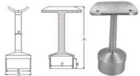
RAIL BRACKET TUBE TOP MOUNT SQUARE, SS304 OR SS316
