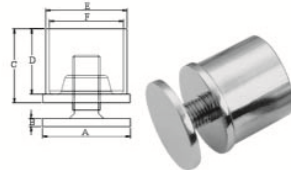
BASE INTERNAL ROUND TUBE, SS304 OR SS316
