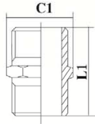
变径六角外螺纹接头 REDUCING HEXAGON NIPPLE(RHN)
