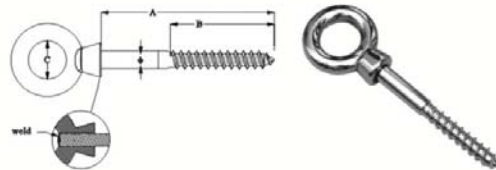
EYE WOODEN SCREW, SS304 OR SS316.
