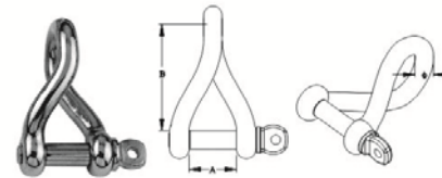
TWIST SHACKLE, SS304 OR SS316. CSXK05
