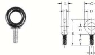
FORGED MACHINERY EYE BOLT S-279 UNC
