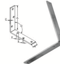
L-SHAPE PLATE, SS304 OR SS316. CB0L
