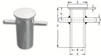
CROSS BOLLARD(系缆桩)
