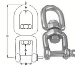
EU SWIVEL EYE AND JAW,SS304 OR SS316. 欧式旋转环
