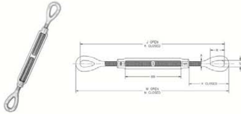
T EYE & EYE TURNBUCKLES HG-226,SS304 OR SS316.
