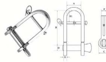
PLATE DEE SHACKLE WITH CROSS BAR,SS304 OR SS316 CSXK0704
