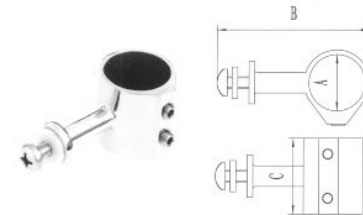
Special Top Slide
