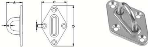
DIAMOND EYE PLATE,SS304 OR SS316. CSMK07
