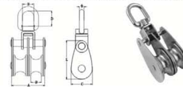
MAME SWIVEL BLOCK(DOUBLE CASTING SHEAVE),SS304 OR SS316.
