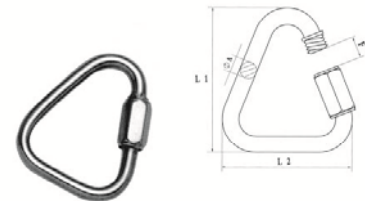
QUICK LINK,SS304 OR SS316,STEEL ELECTRIC GALVANIZED
