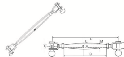
EU CLOSED BODY TURNBUCKLE(欧式封闭花兰螺丝) CSHL03FJ
