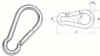
SNAP HOOK WITH SCREW DIN5299 FORM D,SS304 OR SS316,STEEL ELECTRIC GALVANIZED
