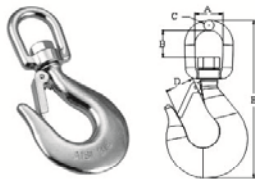
SLIP HOOK--HEAVY TYPE(SWIVEL END WITH SAFETY LATCH),SS304 OR SS316. CSHG08
