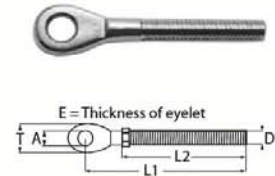
EYE TERMINAL-EXTERNAL THREAD STAINLESS STEEL
