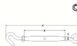
TURNBUCKLE,PIPE(HOOK+EYE),SS304 OR SS316. CSHL03HE
