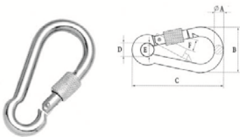
SNAP HOOK WITH EYELET DIN5299 FORM A,SS304 OR SS316,STEEL ELECTRIC GALVANIZED
