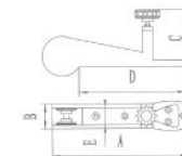
Bow Roller
