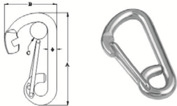
SPRING SNAP-CASTED(HOOK END),SS304 OR SS316.
