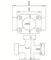
Cross Bollard Single 单十字缆桩
