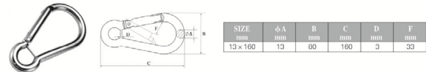
OVAL TYPE SNAP HOOK, STEEL ELECTRIC GALVANIZED
