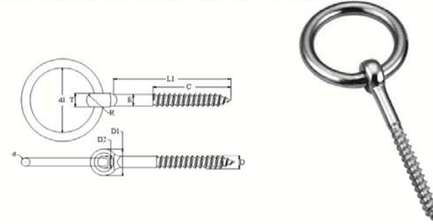
WELDED WOODEN THREADED EYE WITH ROUND RING, SS304 OR SS316.
