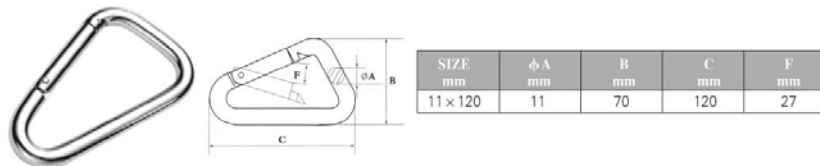
DELTA SNAP HOOK WITH SCREW AND BAR,SS304 OR SS316
