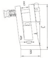
Deck Hinge Angle Base 销式斜山型座
