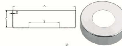
ROUND BASE, SS304 OR SS316
