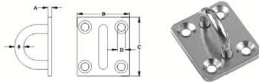
SQUARE EYE PLATE,SS304 OR SS316. CSMK01
