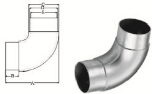
CGWT01 BALUSTRADE ROUND STYLE 90° , SS304 OR SS316
