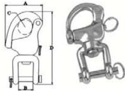
SNAP SHACKLE WITH FORGED SWIVEL JAW,SS304 OR SS316.
