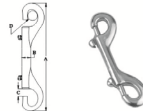
DOUBLE ENDED BOLT SNAP,SS304 OR SS316. CSSH02
