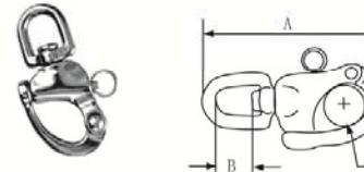
SWIVEL SNAP SHACKLES WITH EYE END(固式旋转弹簧卸扣)
