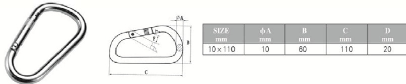
SPRING HOOK WITH FLAT TYPE,SS304 OR SS316
