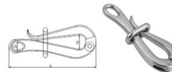
PELICAN HOOK(WITH LINK),SS304 OR SS316.
