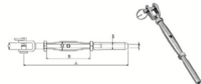
TURNBUCKLE PIPE(WIDE+WIDE TOGGLE),SS304 OR SS316.
