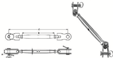
TURNBUCKLE PIPE(WIDE+WIDE TOGGLE),SS304 OR SS316.
