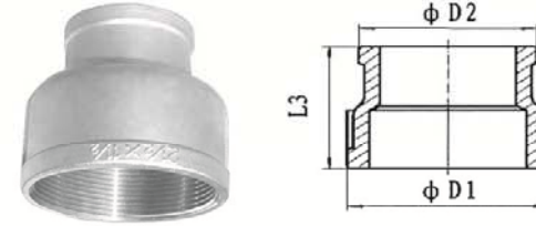
异径有边接头 REDUCING SOCKET BANDED (RSB)
