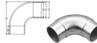
CGWT01 BALUSTRADE ROUND STYLE 90° , SS304 OR SS316
