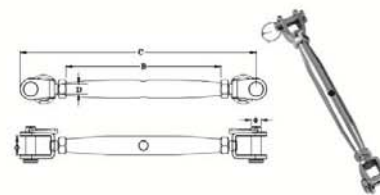
TURNBUCKLE PIPE(JAW+JAW),SS304 OR SS316. CSHL03FJ
