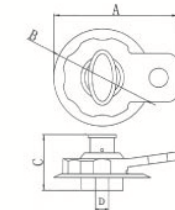
Quick Joint
