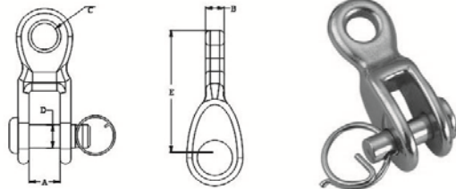
SWAGE TOGGLE,SS304 OR SS316.
