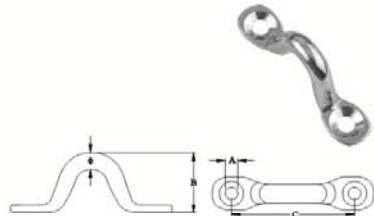
PAD EYE,SS304 OR SS316.CSLB02
