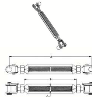
TURNBUCKLE,FRAME TYPE WITH NUT(JAW+JAW),SS304 OR SS316.CSHL03KJ
