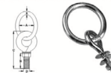
RING BOLT WITH DOUBLE WASHER AND NUT, SS304 OR SS316.
