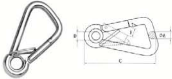
OBLIQUE ANGLE SNAP HOOK WITH EYELET AND RIVETS AT BOTH END,SS304 OR SS316.
