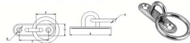
OVAL EYE PLATE(WITH RING),SS304 OR SS316. CSMK04
