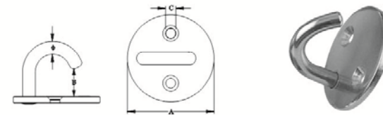
ROUND PLATE(HOOK TYPE),SS304 OR SS316.CSMK01
