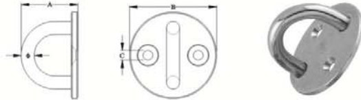
ROUND EYE PLATE,SS304 OR SS316. CSMK05
