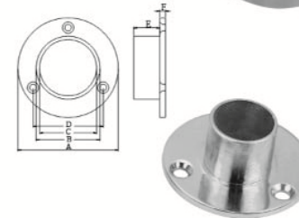
ROUND BASE, SS304 OR SS316
