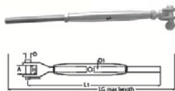
RIGGING SCREW JAW&WIRE ROPE TERMINAL MT FORM STAINLESS STEEL
