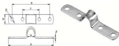
EYE STRAP(FOUR HOLE TYPE),SS304 OR SS316.
