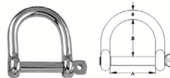
ANCHOR(BOW) SHACKLE(WITH SQUARE HEAD PIN),SS304 OR SS316 CSXK13
