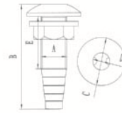
Through Hull Outlets With Hose Connection 出水口
