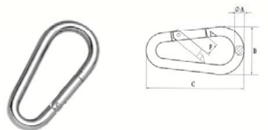
EGG TYPE SNAP HOOK DIN5299 FORM B,SS304 OR SS316,STEEL ELECTRIC GALVANIZED
