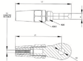
CABLE ENCASING-TUBE, SS304 OR SS316.
