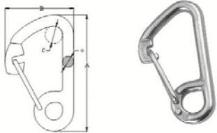
SPRING HOOK,SS304 OR SS316.
