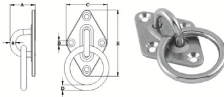
DIAMOND EYE PLATE WITH RING,SS304 OR SS316. CSMK08
